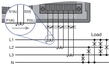
Connection "Current measurement via current transformer"
