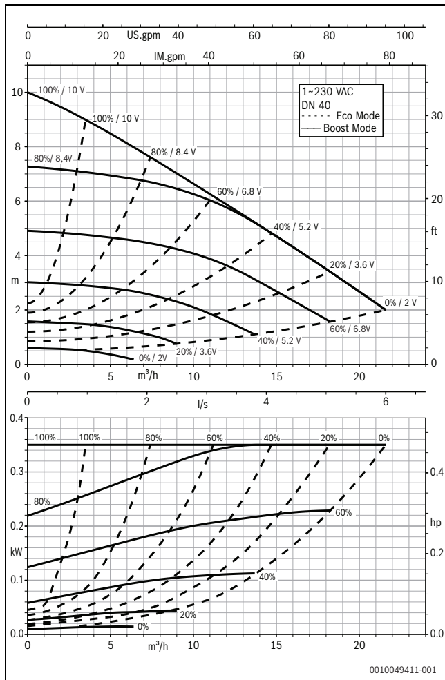
Fig. 11 Pumpekurver Calio 40-100
