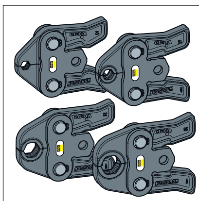
Abb. 9: Pressbacken
