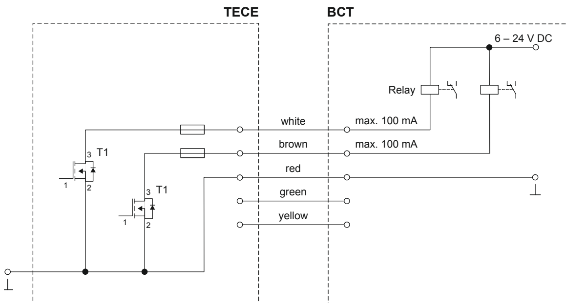
Connection to BCT with external power supply (B)
