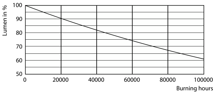
Lumen Maintenance Diagram - MAS LED SON-T IF 3.6Klm 23W 727 E27
